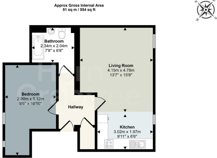
Floorplan
